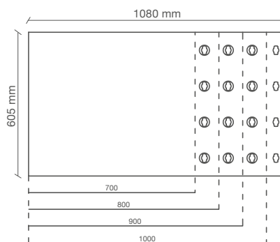
GEOPANEL STAR 70/100
